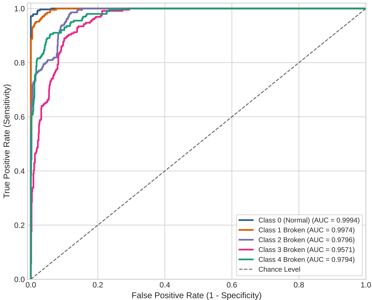
Multi-Class ROC Curves (Real Audio + Telemetry)
